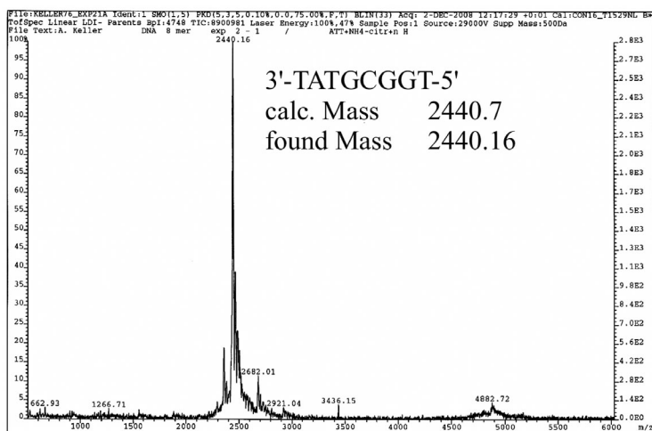
FIG. 9 MALDI-MS spectrum of the modified DNA 8mer after cyanoethyl cleavage
