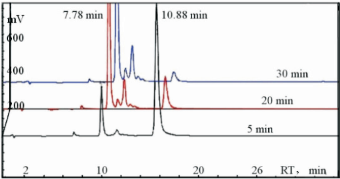
FIG. 3 Stacked RP-HPLC chromatograms illustrating the OH-induced 3'-O-CE cleavage of mono-phosphate 7
