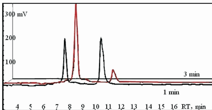
FIG. 5 Stacked RP-HPLC chromatograms for Experiment No. 13 (THF/DMF 1:1)
