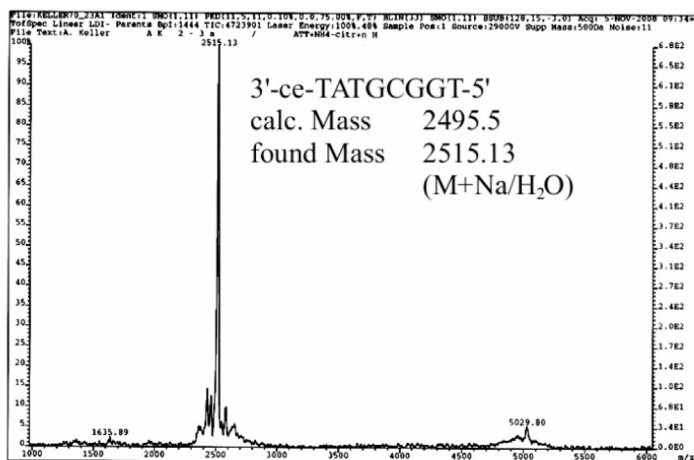
FIG. 8 MALDI-MS spectrum of the modified DNA 8mer with 3'-CE-terminus
