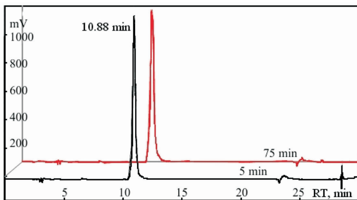
FIG. 4 Stacked RP-HPLC chromatograms of cyanoethyl cleavage experiment under acid conditions
