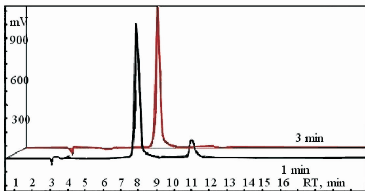
FIG. 6 Stacked RP-HPLC chromatograms for Experiment No. 14 (THF/DMSO 1:1)
