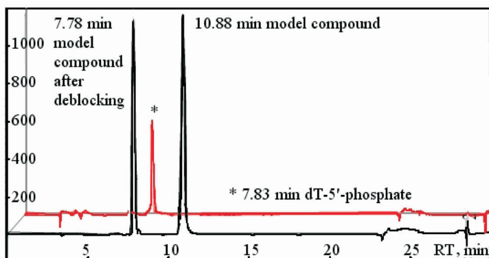
FIG. 2 RP-HPLC chromatogram of model compound 7 and deprotected monophosphate 10
